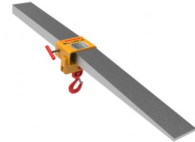
Tandemloc AS24 Series Single Fork Lifting Beams
