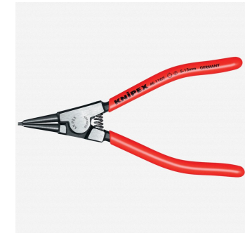
Knipex 46 11 G3 Circlip Pliers for grip rings on shafts 14-18mm
